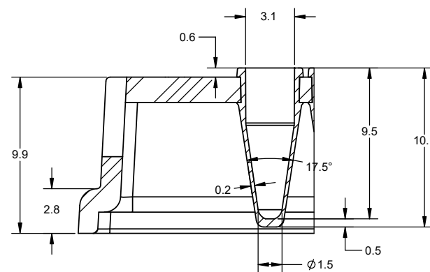
DETAIL W
